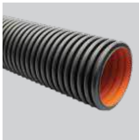
DOUBLE WALL CORRUGATED PLAIN PIPE (ONE COUPLER WITH TWO RUBBER RINGS) (6m) SN8
