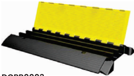
DCPR0003 3 Channel Flexible Cable Protector Size : L900 x W500 x H75 mm Hole Size : L63xH53 mm
